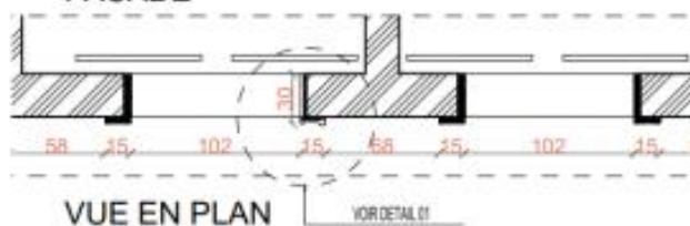
FACADE
