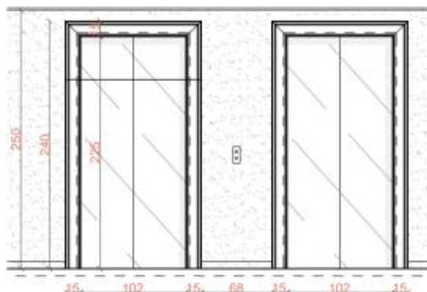
FACADE
